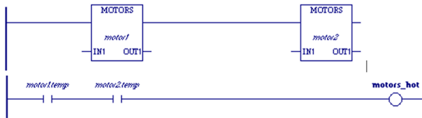
Figure 6 Use of User-Defined Function Block in Ladder Logic
