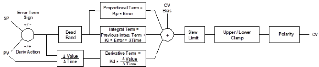
Figure 258: PID_IND Diagram
